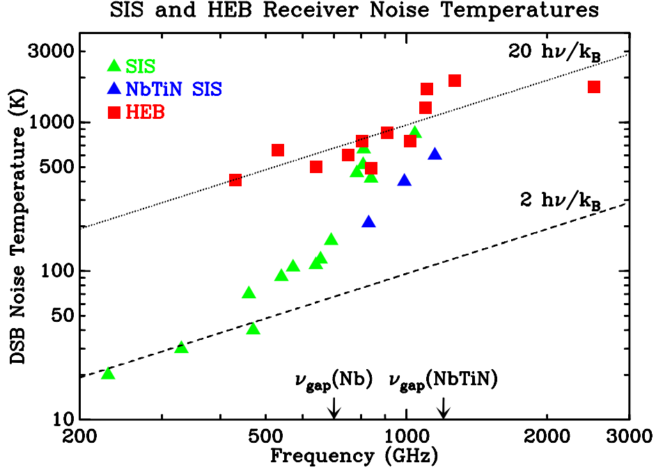
Figure 5: A selection of measured sensitivities for SIS and HEB receivers.
