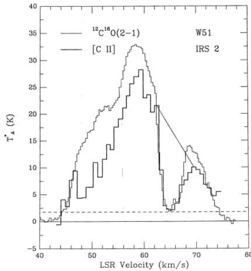
Figure 1: A high-resolution spectrum of the 158 \mu\text{m} [C II] line toward W51 IRS2 [4]. Note the sharp absorption feature, which in this case is most likely produced by a foreground cloud with a low-density PDR.
