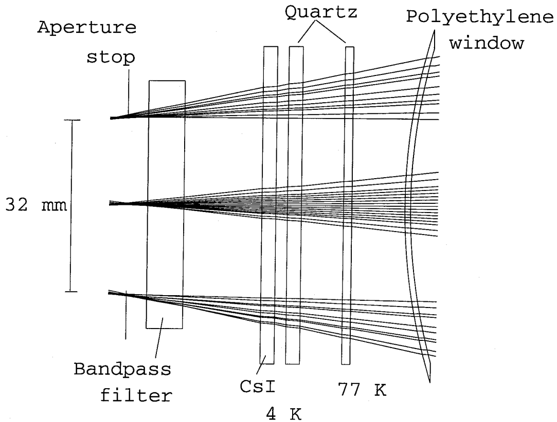
Figure 2.6: The filter arrangement at the entrance of the SHARC cryostat. The filters (and thicknesses) are: high density clear polyethylene vacuum window (1.01 mm); quartz (1.5 mm) with black polyethylene AR coating; quartz (2.5 mm) with a diamond scattering layer on the top and a black polyethylene AR coating on the bottom, Cesium Iodide (2.5 mm) with a clear polyethylene AR coating on both sides; metal-mesh bandpass filter (6.5 mm). The bandpass filters lie in a manually-driven filter wheel with space for four different filters.
