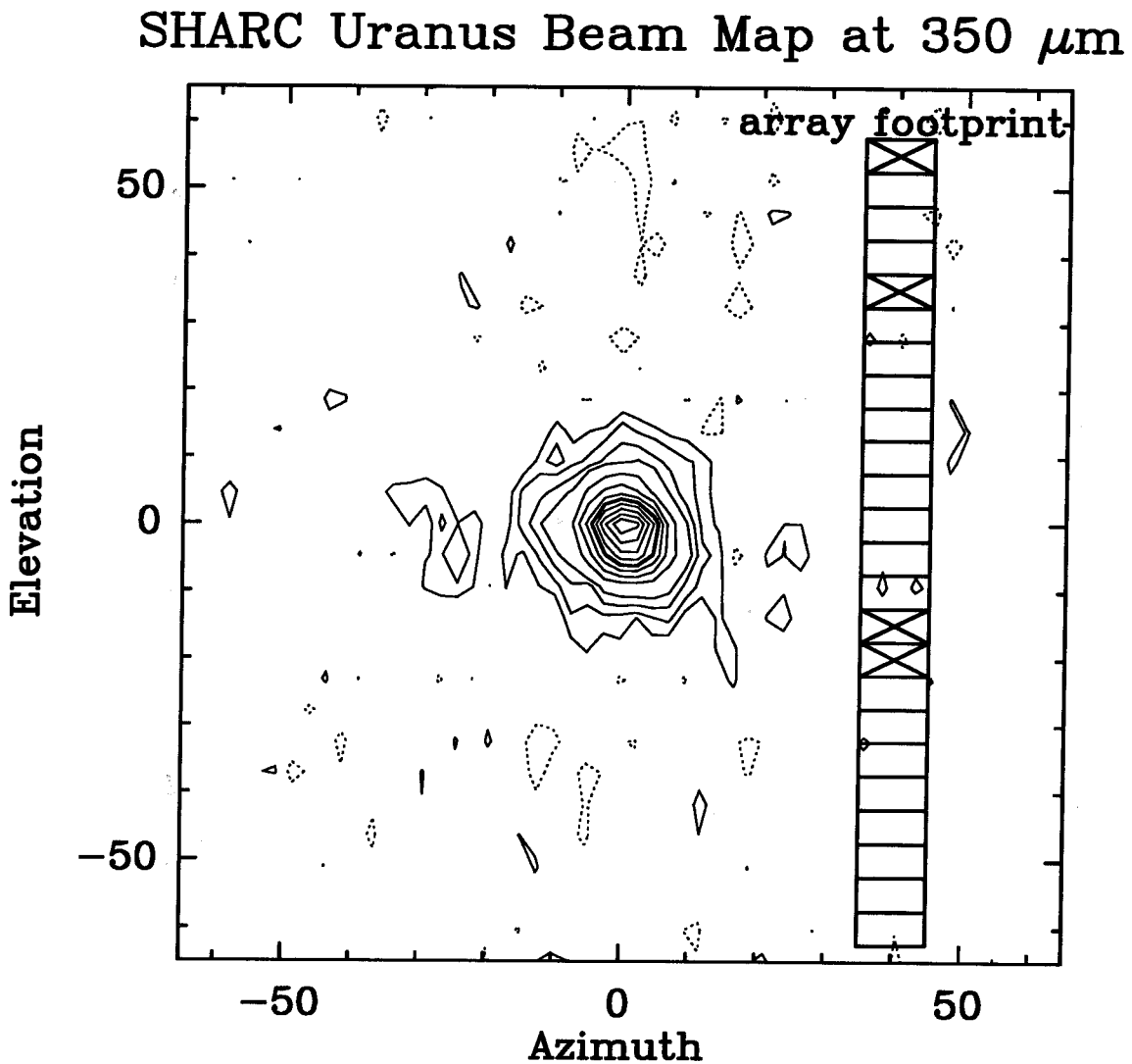
Figure 2.8: A CSO/SHARC beam map at 350 \mu\text{m} constructed from a sum several SHARC scans recorded while the telescope was driven across the planet Uranus at a rate of 3 arcseconds per second. The secondary mirror was chopping 86 arcseconds in azimuth at 4.09 Hz during the scans. The solid contour levels are 2,4,7,10-90% by 10% of the peak flux density. The dashed contour is -2%. The array footprint is shown with non-functioning pixels marked by an X.
