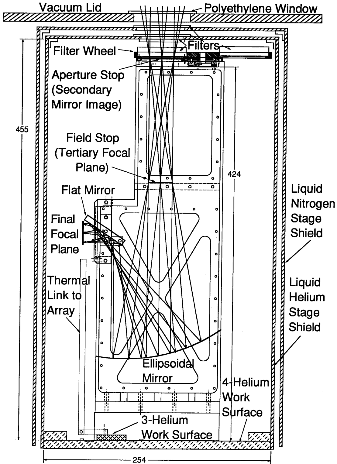
Figure 2.5: A scale drawing of the cryostat optics with dimensions in units of millimeters.
