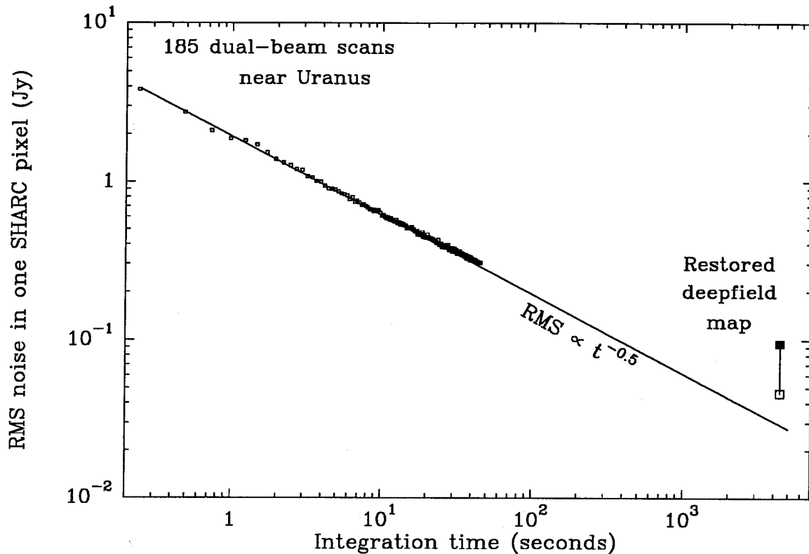
Figure 2.13: The RMS noise in a single SHARC pixel is plotted as a function of integration time at 450\mu\text{m} . The data at the upper left come from raw dual beam scans of Uranus taken within the same hour. The solid square at the right marks the RMS noise achieved in the final restored map of the deep field survey. The open square represents the estimated noise prior to single beam restoration.
