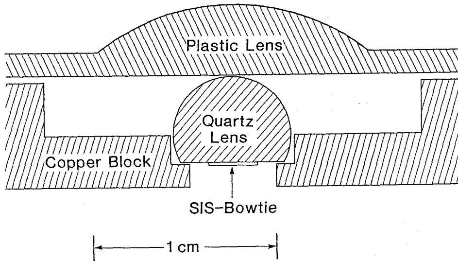
Figure 4.9 Cross section through Bowtie 1. The first mixer block is made so that the quartz hyperhemisphere is located in a hole drilled in the copper mixer block, and held in place by the plastic lens, which is attached to the front of the mixer block. IF connections to the SIS are not shown in this figure.
