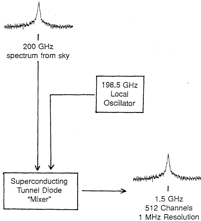
Figure 1.8 Heterodyne detection. Signal radiation at some high frequency \nu_S is combined with a coherent oscillation at frequency \nu_{LO} = |\nu_S - \nu_0| . These are “mixed” by the detector diode so that the spectral information at \nu_S is reproduced at the much lower frequency \nu_0 . This low frequency, or downconverted spectrum can be amplified and analyzed with (relatively) straightforward microwave components.
