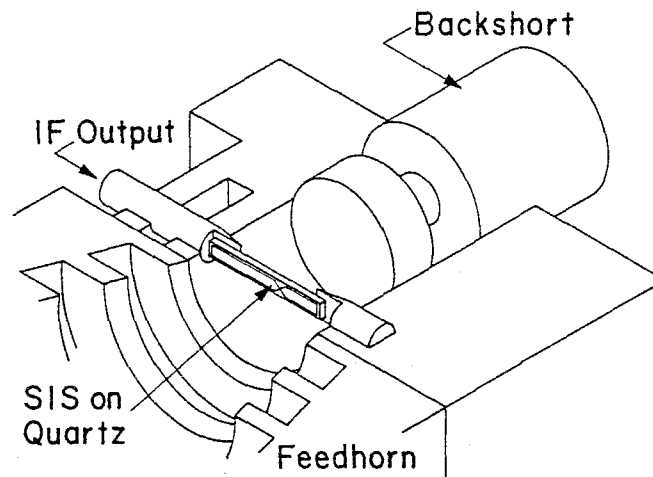
Figure 4.2 Cutaway view of the waveguide-feedhorn mixer block in use at OVRO. The SIS is mounted across a circular waveguide. The waveguide diameter is 2.4 mm, about equal to the free space wavelength of the radiation it will detect. A movable short in the waveguide behind the SIS improves the coupling efficiency between the waveguide and the SIS. A feedhorn efficiently transforms the waveguide radiation to a Gaussian profile free space beam. (Woody, Miller and Wengler, 1985).
