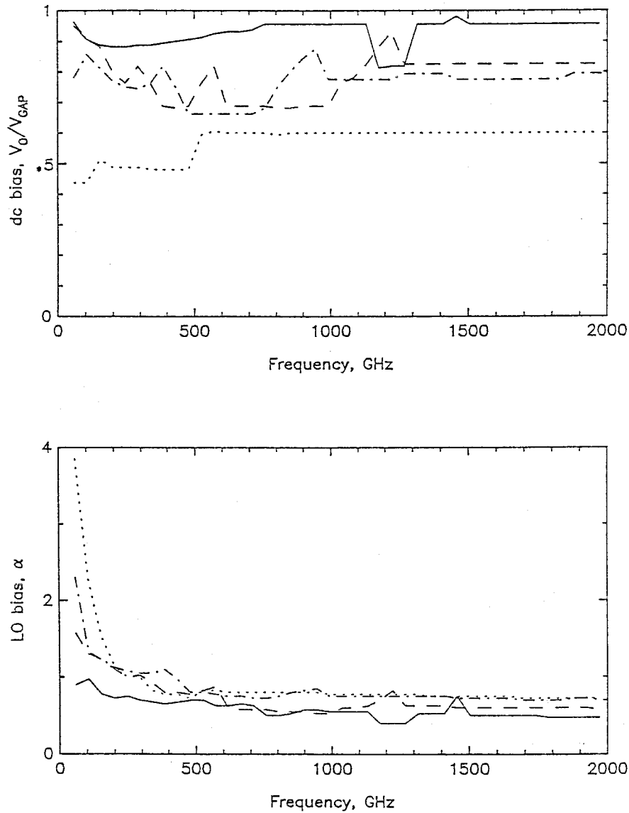
Figure 3.11 Optimum bias vs. frequency. The dc and LO voltages which optimize T_R for the four junctions of fig. 3.1 are plotted. a) The dc bias voltage. b) The LO voltage, shown in terms of the Bessel function argument \alpha = eV_{LO}/\hbar\omega_{LO} .
