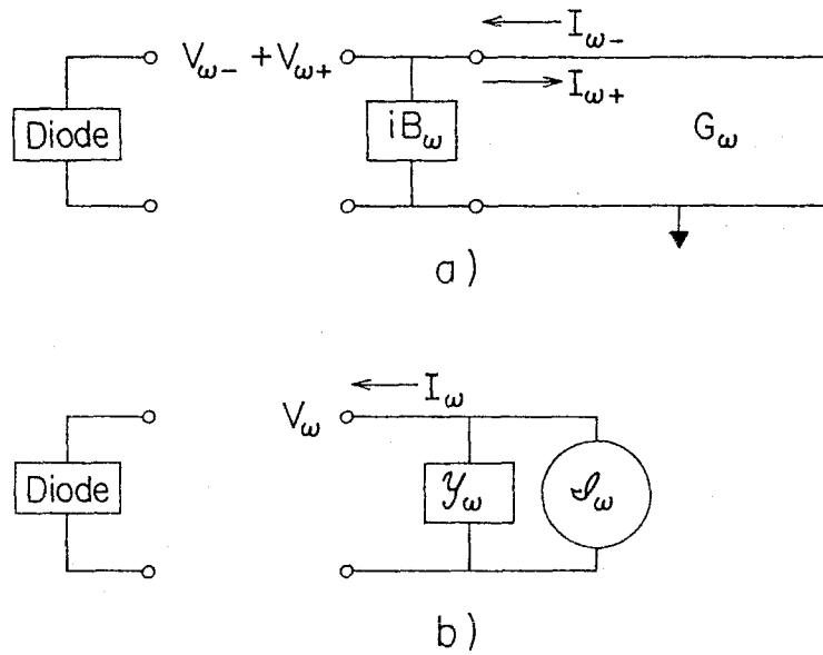
Figure 2.1 External circuit. a) The external circuit of the mixer is represented by a semi-infinite transmission line. Reactance from the external circuit appears as a lumped component at the line terminals. The direction of positive current flow for the - and + going waves are shown. b) An equivalent circuit which is usually used in mixer theories. A linear admittance shunted by a perfect current source models the circuit at each frequency.
