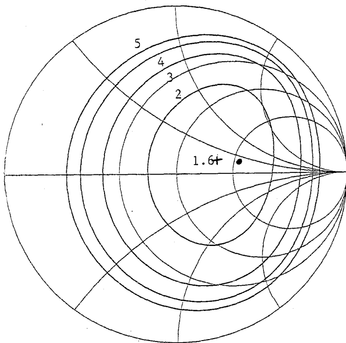
Figure 3.3 Mixer noise vs. \mathcal{Y}_S . Mixer noise is shown as contours of constant N_M . The calculations are done for junction 2 at frequency .1\nu_{\text{GAP}} = 130.5 GHz, assuming \mathcal{Y}_S = \mathcal{Y}_I . Minimum N_M is shown with a +, Y_{\text{LO}} is shown with a •.
