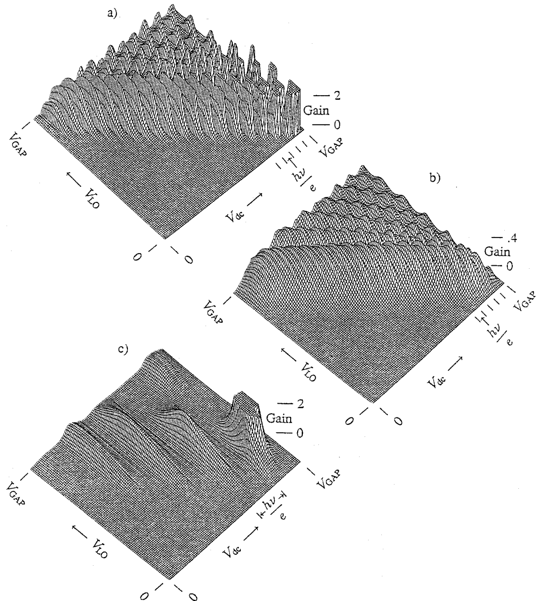
Figure 3.2 Conversion gain vs. dc and LO voltage bias. a) Junction 1 from fig. 3.1 operated at frequency .025\nu_{GAP} = 37 GHz. Gain is clipped at 2. b) Junction 2 operated at frequency .025\nu_{GAP} = 32.6 GHz. The gain scale in this case is 5 times lower than for a) or c). c) Junction 2 at a higher frequency, .1\nu_{GAP} = 130.5 GHz. Gain is clipped at 2.
