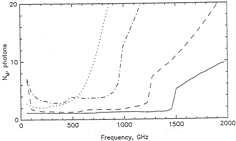
Figure 3.10 Mixer noise, N_M , vs. frequency for the four junctions of fig. 3.1.
