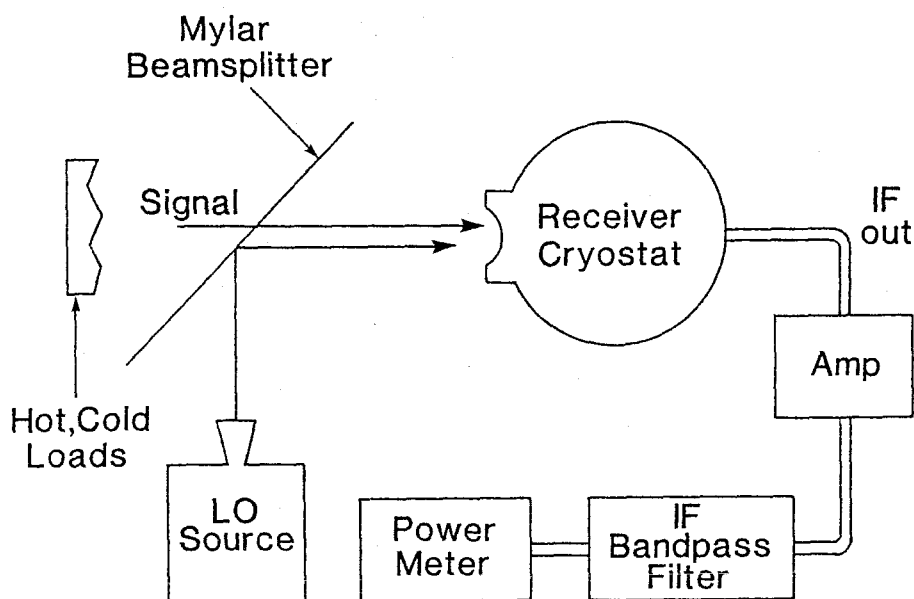
Figure 4.12 Receiver test set-up. The LO is combined with the test signal by partial reflection from a 25\ \mu\text{m} thick mylar sheet. The SIS-bowtie mixer and the first IF amplifier are in the receiver cryostat. The mixer output is further amplified and filtered outside the cryostat, and then measured with a power meter.
