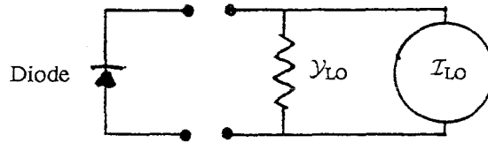
Figure 1.4 RF Circuit for a diode power detector. The power source is represented by an harmonic current source with angular frequency \omega_{LO} , shunted by an admittance \mathcal{Y}_{LO} , which is called the source admittance.
