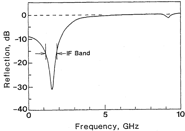
Figure 4.8 Reflection coefficient of IF circuit. The transformation properties of the IF circuit are verified by measuring reflection return loss from the mixer with a 100\ \Omega chip resistor in place of the SIS. The design IF band is centered at 1.5 GHz.
