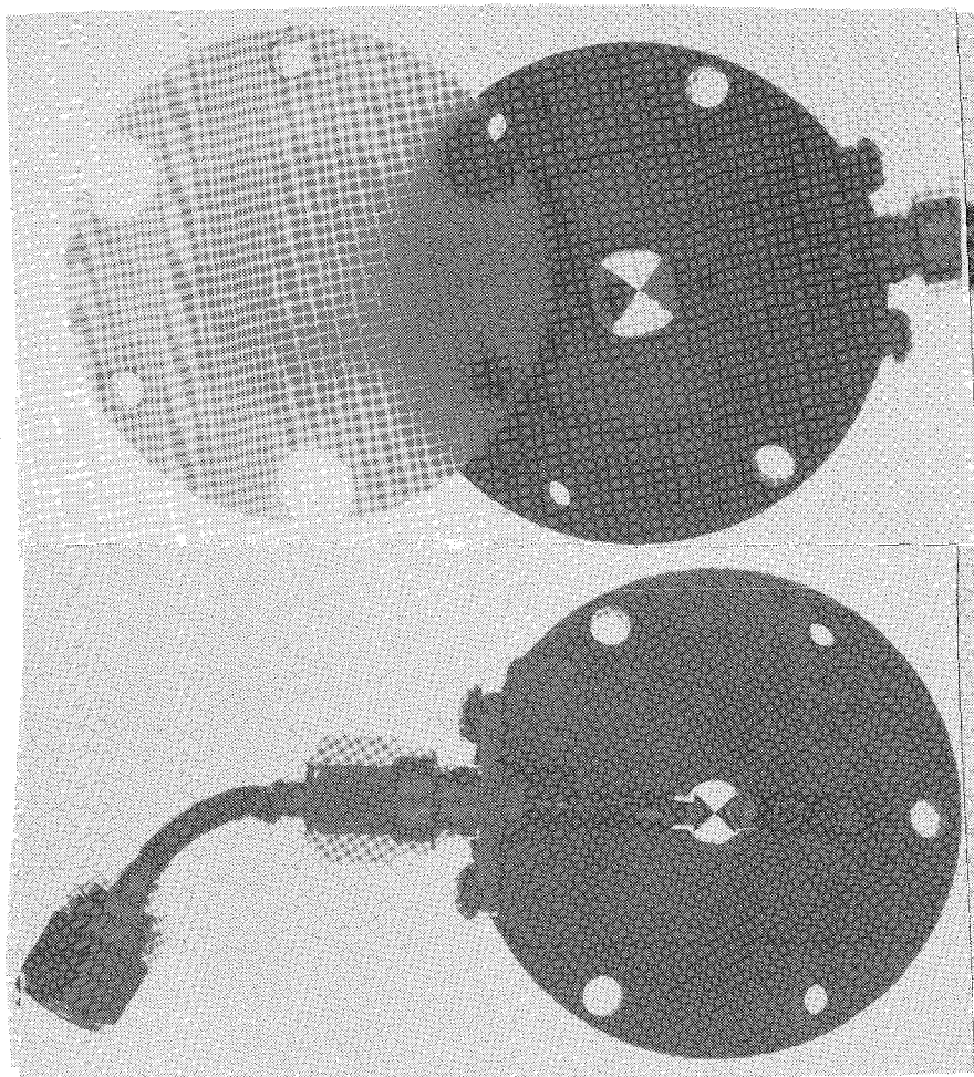
Figure 4.10 Photographs of Bowtie 1. (a) From the RF side, the plastic lens is shown out of place so that the SIS-bowtie can be seen through the fused quartz hyperhemisphere. (b) From the other side, the ground and IF connections to the SIS-bowtie can be seen. These connections are made from springy metal to hold the SIS against the hyperhemisphere.
