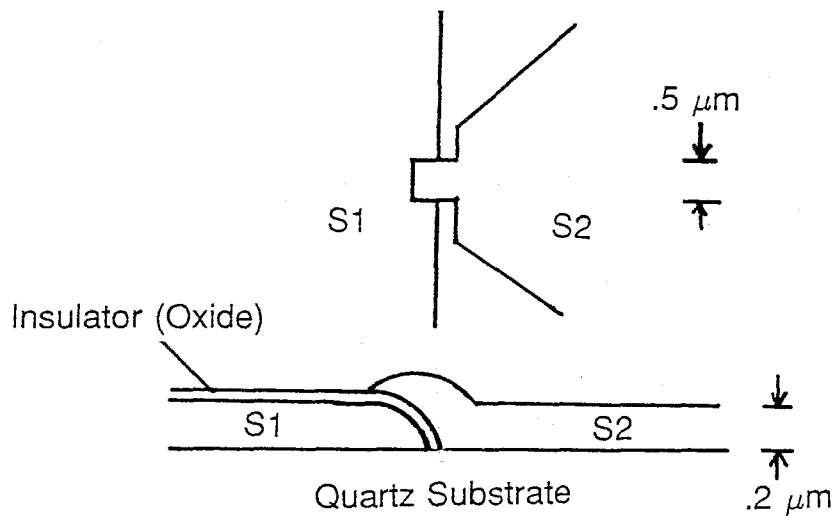
Figure 4.3 Schematic view of SIS junction. At the top is shown the view looking down onto the junction. Below is shown a cross-section through a junction (not to scale). The current path is from S1, through the insulator, to S2.
