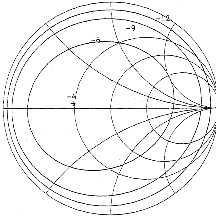
Figure 3.8 Gain vs. \mathcal{Y}_S at a lower frequency. Available gain, labeled in dB, is calculated for junction 2 at a frequency .025\nu_{\text{GAP}} = 32.6 GHz, keeping \mathcal{Y}_S = \mathcal{Y}_I . The maximum available gain point is shown by a +.
