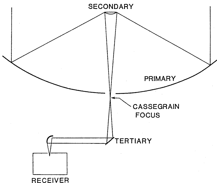
Figure 4.21 Optics on 10.4 m telescope at OVRO. The extreme rays traced are for the -13 dB contour of the Gaussian beam for which the optics are designed.
