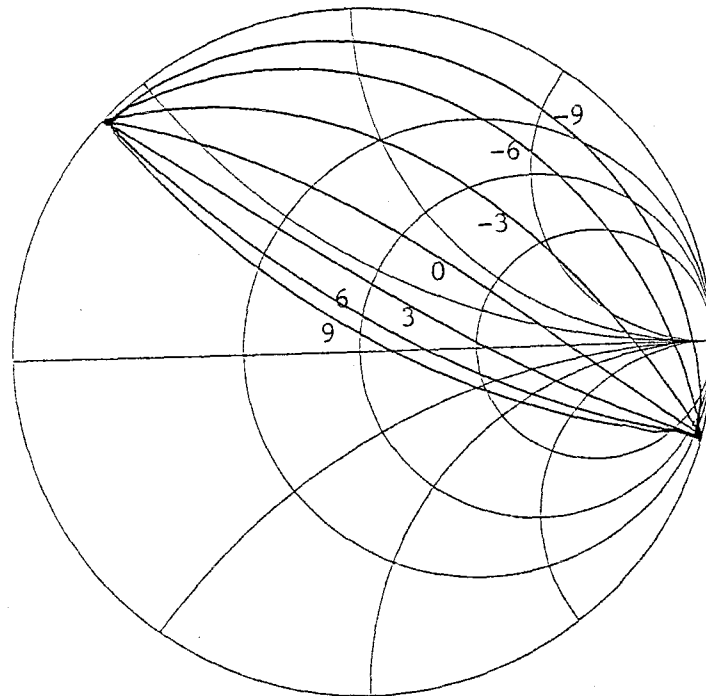
Figure 3.4 Mixer gain vs. \mathcal{Y}_S for the DSB mixer. Gain is shown in contours of constant G_{01} , expressed in dB. The calculations are done for junction 2 at frequency .1\nu_{\text{GAP}} = 130.5 GHz, assuming \mathcal{Y}_S = \mathcal{Y}_I . The lower left half of the Smith chart, with no contours of gain in it, is the region in which infinite gain is available from the mixer.
