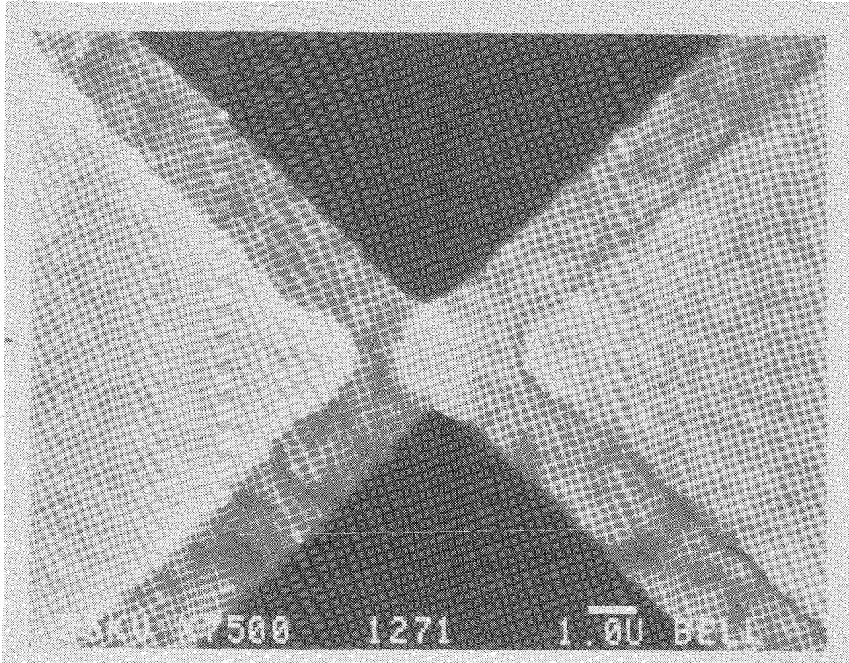
Figure 4.4 Micrograph of an SIS-Bowtie. A scanning electron micrograph of an SIS-Bowtie shows the overlapping superconductors which form the SIS, and the small scale part of the bowtie antenna. The bowtie shape is accurately maintained down to about 1 \mu\text{m} scale size.
