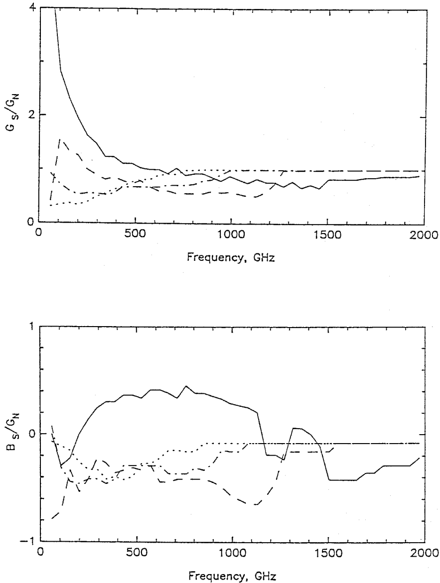
Figure 3.12 Optimum signal source admittance vs. frequency. The real and imaginary parts of \mathcal{Y}_S = G_S + iB_S , which result in minimum T_R are plotted for the four junctions of fig. 3.1. a) The real part, normalized to G_N . b) The imaginary part, similarly normalized.
