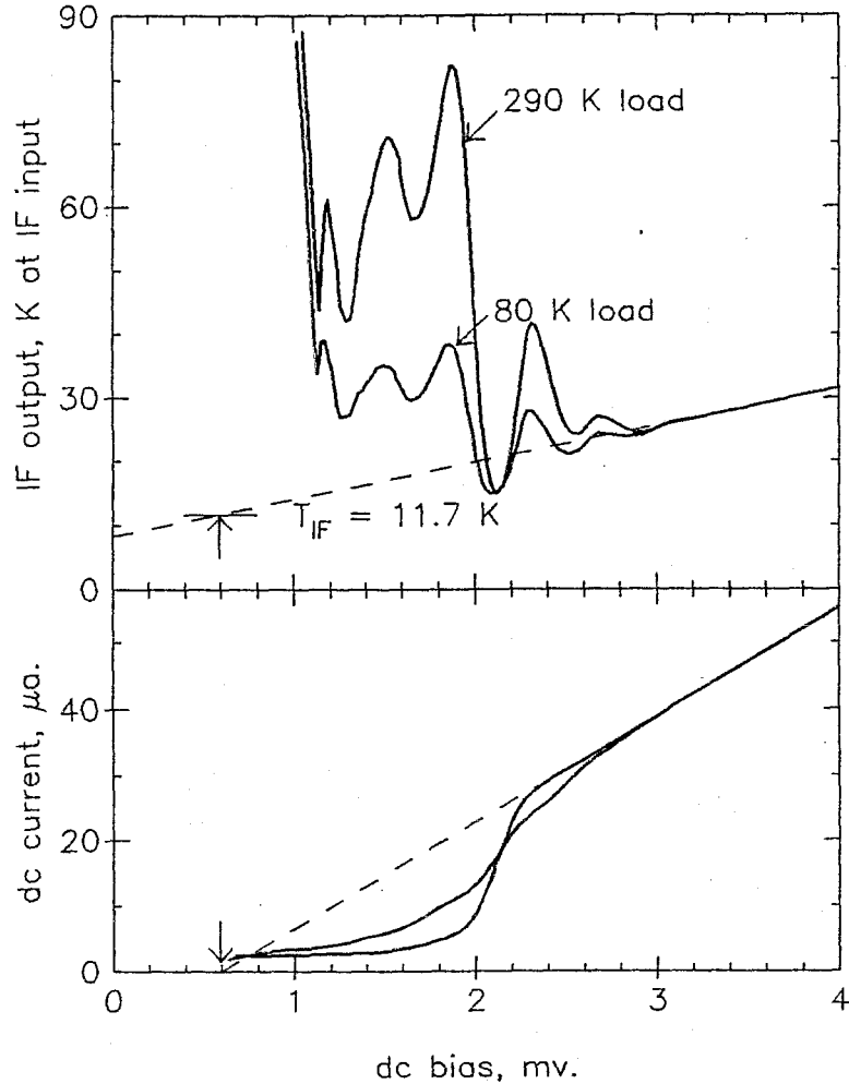
Figure 4.14 I - V and IF power vs. dc bias voltage. Below 3 mV, heterodyne response is seen, this is for a waveguide mixer at 95 GHz (Woody, Miller and Wengler, 1985). Above 3 mV, there is no heterodyne response, and the SIS shot noise is used to calibrate the IF amplifier chain as described in the text.
