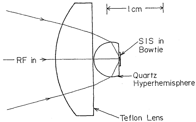
Figure 4.1 Bowtie mixer optics. An SIS junction is fabricated integrally with a planar bowtie antenna, on a thin quartz substrate. This is placed on the flat surface of a quartz hyperhemisphere. Radiation incident on the plastic lens is focussed into the quartz hyperhemisphere, which further focuses the beam into the center of the bowtie antenna. The radiation is thus coupled to the SIS, which is at the center of that bowtie.
