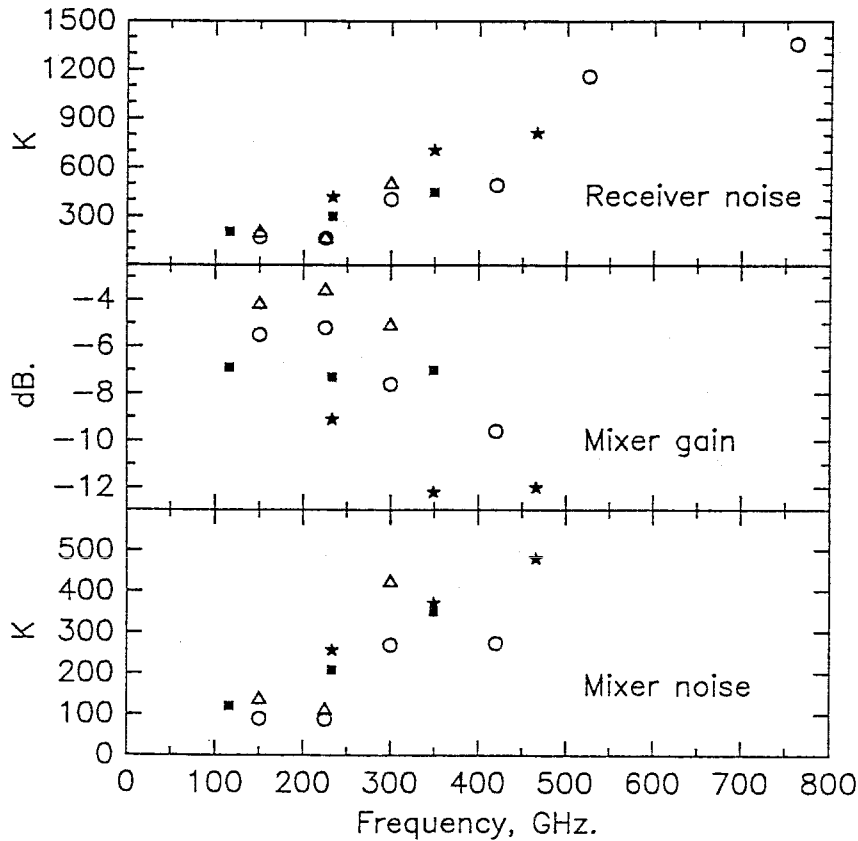
Figure 4.17 Mixer and receiver double sideband performance vs. LO frequency. * – Bowtie 1 with magnetic field applied. ■ – Bowtie 1 with no magnetic field. △ – Bowtie 2 with no magnetic field. ○ – Bowtie 2 with magnetic field. These are the same data as in tables 4.2 and 4.3.
