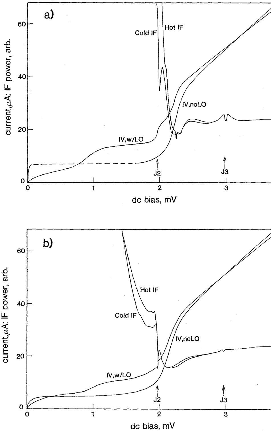
Figure 4.15 I-V and IF power at 466 GHz in Bowtie 1. a) With no magnetic field applied, the IF power rises quickly as the dc bias is lowered, reliable heterodyne results seem unlikely. b) With magnetic field applied, there is a flat region in the IF power curve in which heterodyne response can be accurately measured. The voltages marked J2 and J3 are where the ac Josephson frequency is respectively twice and three times the LO frequency.
