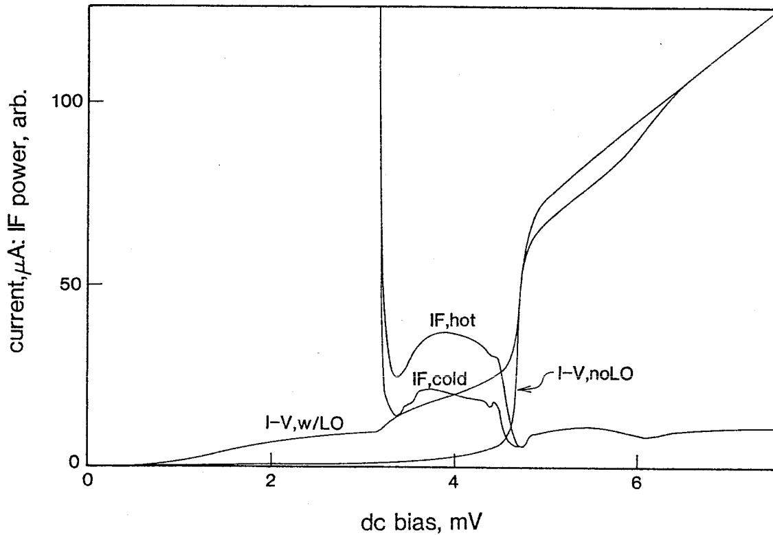
Figure 4.16 I - V and IF power at 225 GHz in Bowtie 2. The IF power is measured with a small magnetic field applied. A broad, flat region of heterodyne response is seen above the high IF power region associated with chaotic noise in the SIS.
