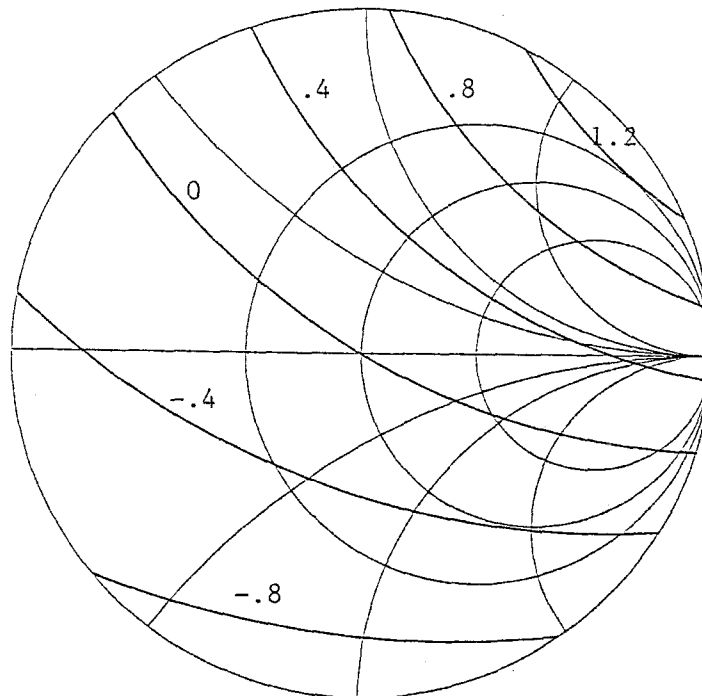
Figure 3.5 Mixer IF output admittance vs. \mathcal{Y}_S . The contours are labeled with the normalized output admittance, G_{\text{IF}}/G_N . Calculations are done using junction 2 at frequency .1\nu_{\text{GAP}} = 130.5 GHz, assuming \mathcal{Y}_S = \mathcal{Y}_I .
