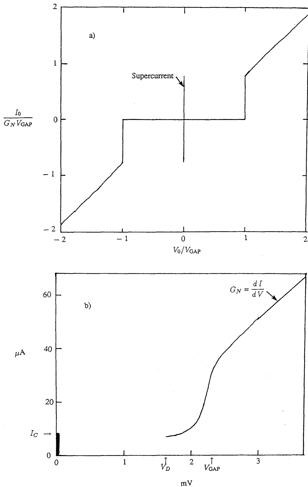
Figure 1.3 SIS dc I - V curve. a) The I - V calculated for an SIS at 0 K, using BCS theory. b) A measured I - V for an imperfect SIS at 4.5 K. Features such as the supercurrent, I_C , the gap voltage V_{GAP} , the normal state admittance G_N , and the dropback voltage V_D are shown.
