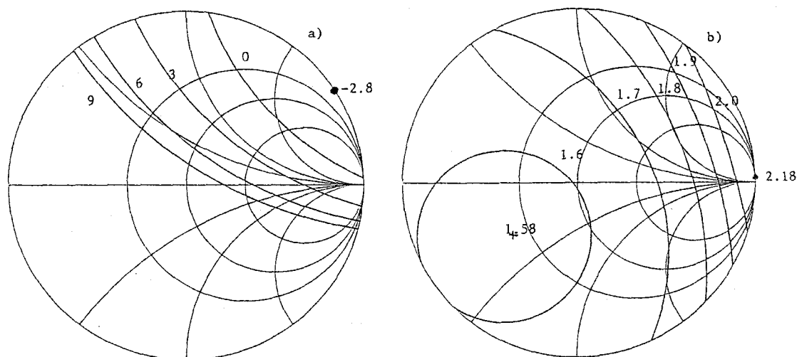
Figure 3.6 Mixer performance vs. \mathcal{Y}_I , for \mathcal{Y}_S fixed. The calculations are done using junction 2 at frequency \nu_{\text{GAP}} = 130.5 GHz. a) Available gain in dB vs. \mathcal{Y}_I . Infinite gain is available for \mathcal{Y}_I in the lower left half of the Smith Chart. The minimum gain point of -2.8 dB is shown by a \bullet . b) Mixer noise in photons, N_M , vs. \mathcal{Y}_I . Minimum noise occurs at the point shown with a + , maximum noise occurs at the point labeled with a \bullet .
