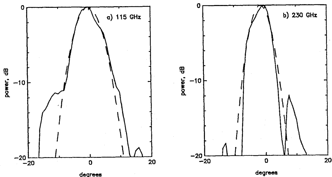
Figure 4.6 Bowtie mixer E-plane beam patterns. The solid lines show the measured E-plane patterns of Bowtie 2. The dashed lines show Gaussian profiles which match the patterns at their half power points. a) Measured at 115 GHz. The full angle between half power points is 8.6^\circ . b) Measured at 230 GHz. The full angle between half power points is 6.7^\circ .
