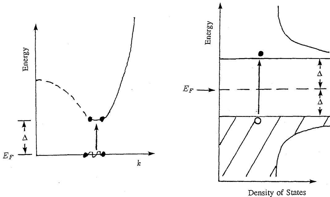
Figure 1.1 BCS superconductor electronic states. a) The pair states are all at the Fermi Energy. The quasiparticle excitation dispersion curve is shown with a broken pair occupying it (Barone and Paterno, 1982). The minimum quasiparticle excitation energy is \Delta . b) In the semiconductor picture, the quasiparticle states are divided into a conduction-like and a valence-like band. A broken pair in this picture is represented by promoting a valence-like particle into the conduction band.
