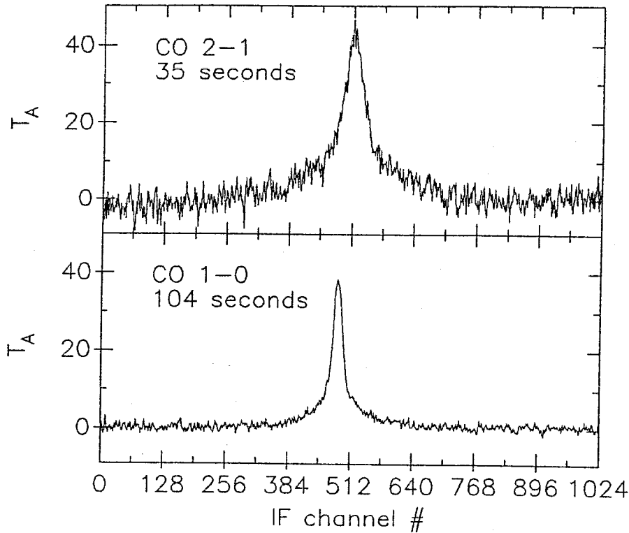
Figure 4.20 Two CO transitions in Orion measured with bowtie-SIS. The data are in 1024 channels spaced .5 MHz apart. The center channel corresponds to line frequencies of 230.531 GHz for the J=2-1 transition and 115.268 GHz for J=1-0. Signal was integrated for the times shown.
