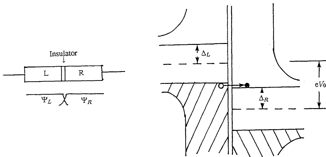
Figure 1.2 SIS tunnel junction. a) The diode consists of two superconductors, L and R , separated by a very thin insulator. Electronic wave functions, \Psi_{(L,R)} , overlap in the insulator. b) The semiconductor picture of an SIS, with a dc voltage V_0 applied, showing one quasiparticle tunneling.
