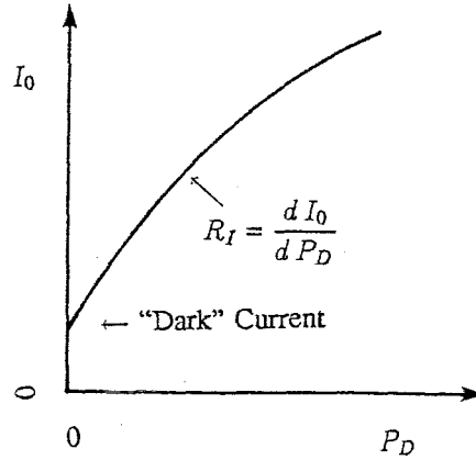
Figure 1.5 Photo-current response of a diode. At a constant dc voltage bias, the dc current through the diode is plotted as a function of the rf power absorbed in the diode. At low powers, the response is linear. The detection mechanism is rectification of the rf waveform.
