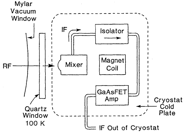
Figure 4.13 Receiver cryostat. RF passes through a mylar vacuum window and a Quartz window at 100 K on its way to the bowtie mixer. The mixer, and the first stages of IF amplification are mounted on the cold plate of this liquid helium cryostat.
