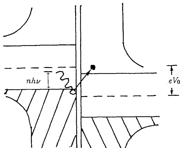
Figure 1.7 Photon-assisted-tunneling in an SIS. The simultaneous absorption of n photons can cause current to flow when eV_0 + nh\nu > eV_{\text{GAP}} .
