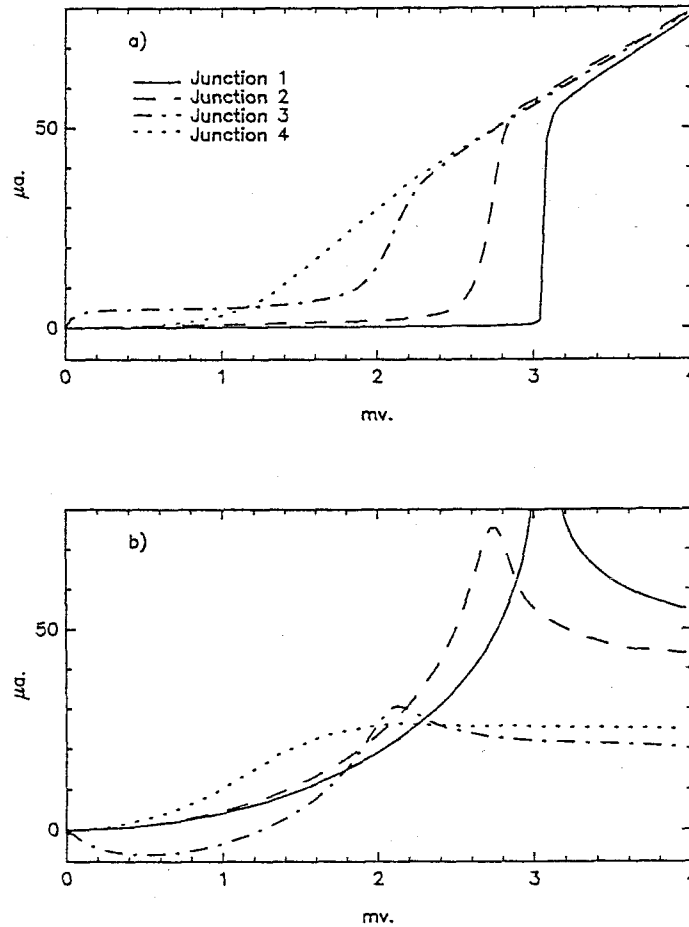
Figure 3.1 Complex response function, j , for four tunnel diodes. a) \text{Im } j is the measured I-V of each diode. b) \text{Re } j is the numerically determined Kronig-Kramers transform of \text{Im } j .
