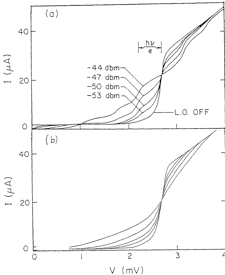
Figure 1.6 SIS I - V s with applied rf. a) The I - V measured with no rf and with four different rf power levels of 115 GHz radiation. Photon steps in the I - V are clearly seen. b) Predictions of the I - V with incident rf from the classical theory described in the previous section. Photon steps cannot be predicted with the classical theory.
