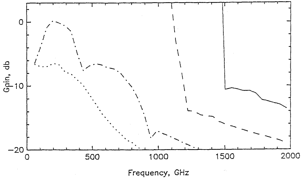
Figure 3.9 Gain vs. frequency for four tunnel junctions. The available gains for the four junctions of fig. 3.2 are shown as LO frequency is varied. At low frequencies, the available gains for junctions 1 and 2 are infinite, and therefore do not appear in the figure.
