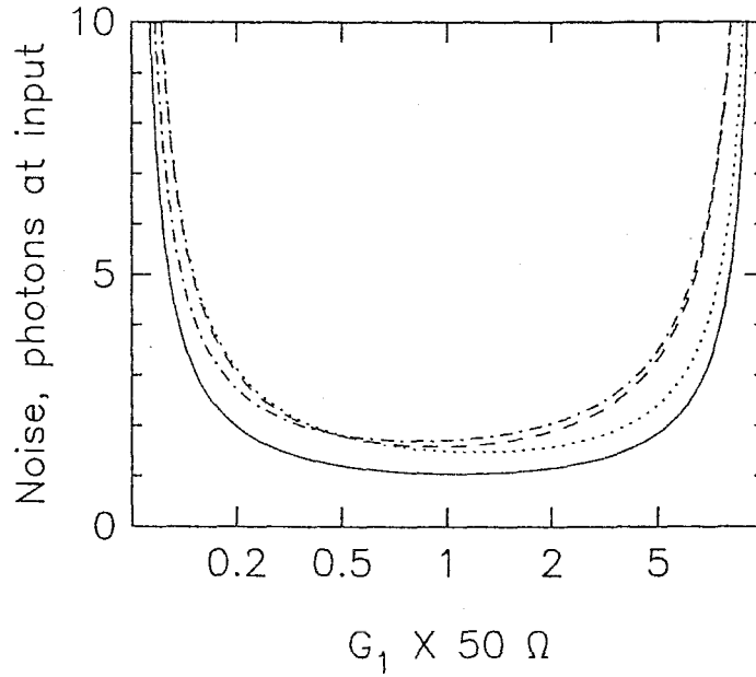
Figure 2.2 Mixer noise N_M vs. real source admittance G_1 for a nearly ideal SIS with large LO power. The a) dashed, b) dotted and c) dash-dot lines are for image termination equal to a) signal termination, b) open circuit, and c) short circuit. The solid line is a plot of (2.6.1) for comparison. The x-axis is the zero reactance slice through a standard Smith chart.
