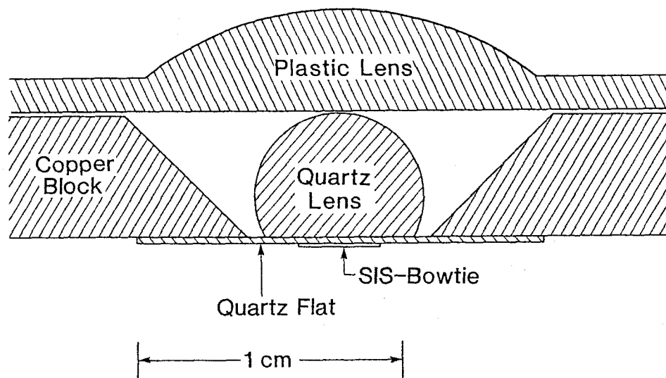
Figure 4.11 Cross section through Bowtie 2. The hyperhemisphere in this mixer is glued to a thin quartz flat, which is indium-soldered to the copper mixer block.
