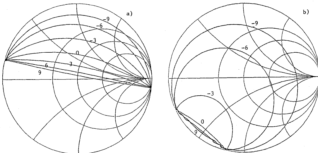
Figure 3.7 Gain vs. \mathcal{Y}_S for two different junctions. Gain contours are labeled in dB. a) Junction 1 at frequency .1\nu_{\text{GAP}} = 148.0 GHz. Infinite gain is available for \mathcal{Y}_S in the lower half of the Smith chart. b) Junction 3 at frequency .1\nu_{\text{GAP}} = 103.2 GHz. Large but finite gain is available for \mathcal{Y}_S in only a very small area at the lower left of the Smith chart.
