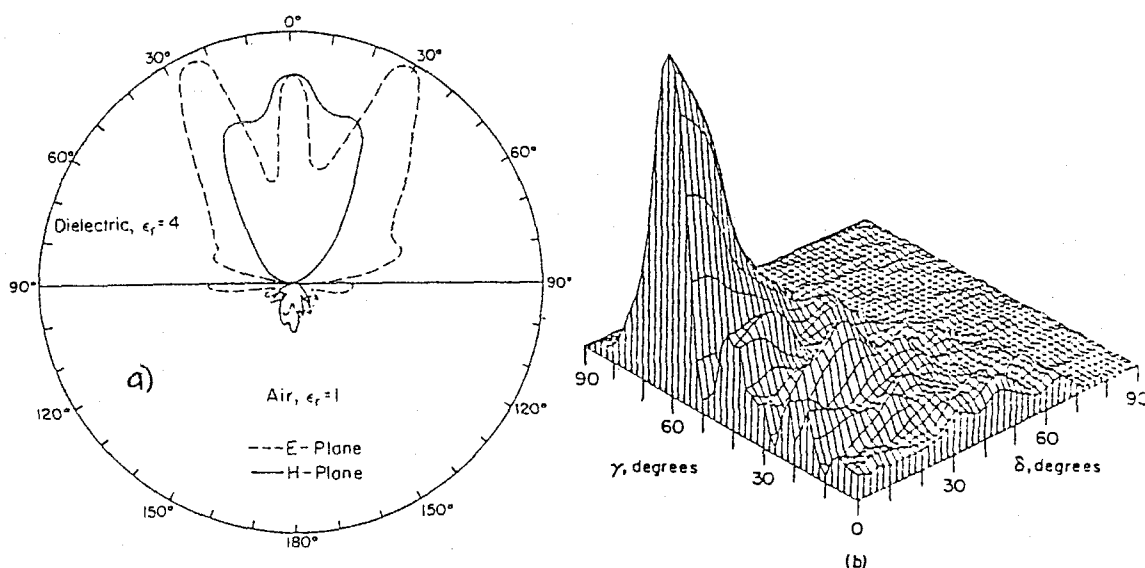
Figure 4.5 Bowtie antenna patterns. a) Pattern measured at 10 GHz on a scale model of an imaging array (Rutledge and Muha, 1982). b) Pattern measured for a single bowtie at 94 GHz (Compton et al. , 1987). The zero of the \gamma and \delta axes show degrees away from the normal in the E-plane and H-plane of the bowtie respectively. Only one quadrant of the pattern is shown, since the other three are simply related to this by the symmetries of the antenna.
