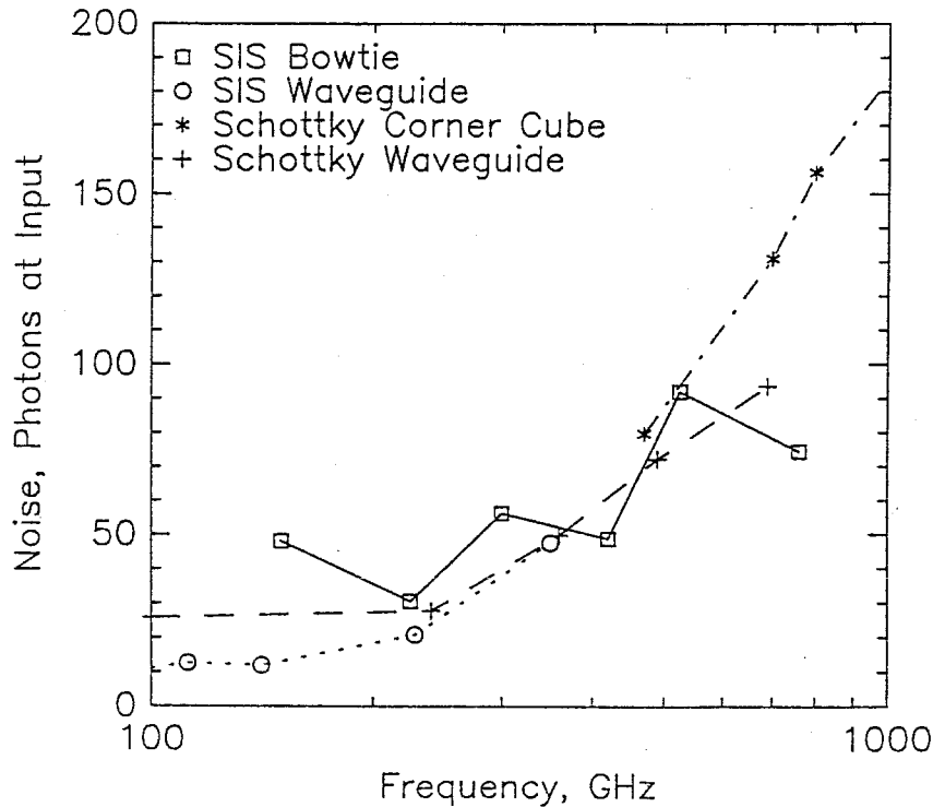
Figure 4.19 Comparison of receiver noises for different technologies. Each waveguide point is measured in a different receiver. The SIS bowtie numbers are from a single receiver (Bowtie 2). The Schottky corner cube numbers are from a single receiver (Betz, 1987; Zmuidzinas, 1987). Each Schottky waveguide datum is from a different receiver (Predmore et al. , 1984; Erickson, 1985 & 1987). Each SIS waveguide datum is from a different receiver (Räsänen et al. , 1986; Pan et al. , 1983; Ibruegger et al. , 1984; Ellison and Miller, 1987; Theis DeGrauw, private communication).
