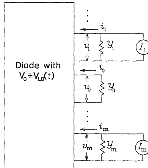
Figure 1.9 Schematic diagram of the equivalent circuit for a mixer diode heterodyne receiver. The LO pumped diode is represented by a multi-port linear network. Each port corresponds to a different sideband. The circuit to which the diode is attached is represented by an admittance \mathcal{Y}_m at each sideband port. A current source I_m accounts for any noise or signal power incident on the diode at that frequency.
