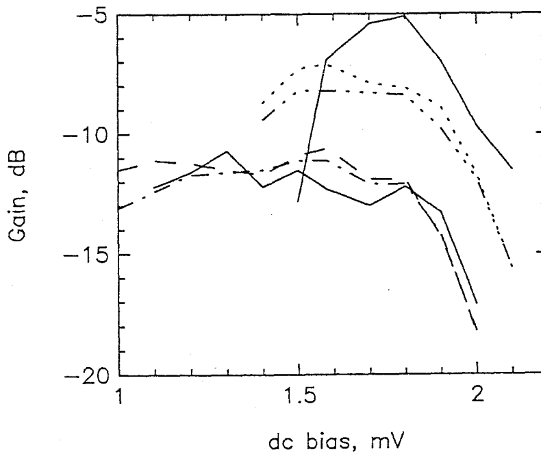
Figure 4.18 Gain measured with sidebands. The measurements were made using Bowtie 1 at an LO frequency of 350 GHz. The dashed line is measured with cold load and magnetic field. The dot-dash line, with hot load and magnetic field. Dotted line, with cold load, no magnetic field. Dash-dot-dot-dot line, with hot load, no magnetic field. The lower and upper solid curves are the gains inferred from hot/cold load measurements, with and without magnetic field, respectively.
