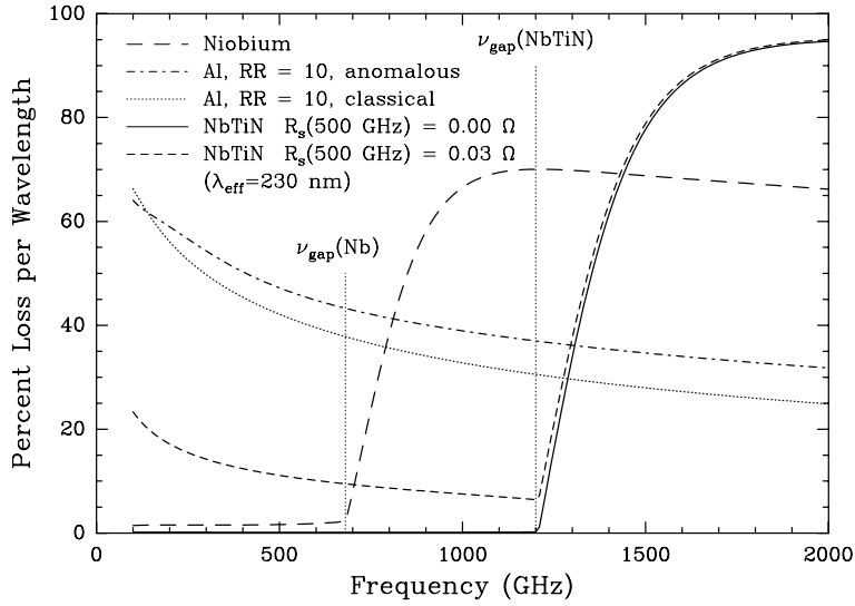
Figure 3. Calculated losses for thin-film microstrip transmission lines used in SIS mixer tuning circuits for various conductors, including NbTiN. The microstrip width is 5\ \mu\text{m} , and the dielectric is 400\ \text{nm} SiO ( \epsilon = 5.6 ).
