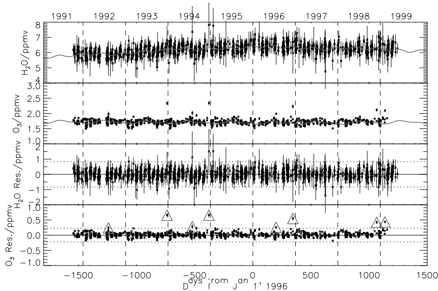
Figure 6. O 3 and H 2 O atmospheric abundances (volume mixing ratio in ppmv; 1ppmv = 10 -6 ) at 55 km (1991-1999) from UARS/HALOE satellite measurements between 30° South and 30° North. Upper two curves show the rough data for H 2 O and O 3 respectively, with the regression model (sinusoidal curve) superimposed. The lower two curves display the residuals (measurements minus model) after having removed the expected long term variations. Dotted lines indicate the 3σ level. Data points above this level are shown by triangles.
