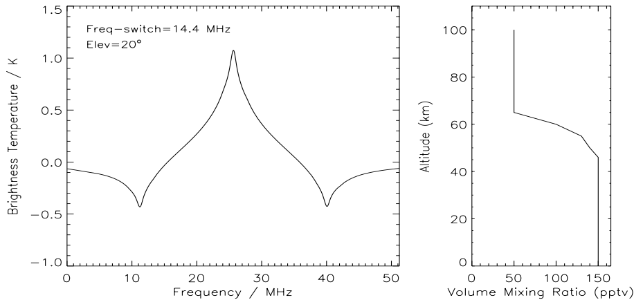
Figure 4. Simulation with MOLIERE of a CSO spectrum and the associated reference HCN volume mixing ratio profile ( 1\text{pptv} = 10^{-12} ) used for the computation (here the same profile than the "MOLIERE: A priori" HCN profile plotted in Figure 1).
