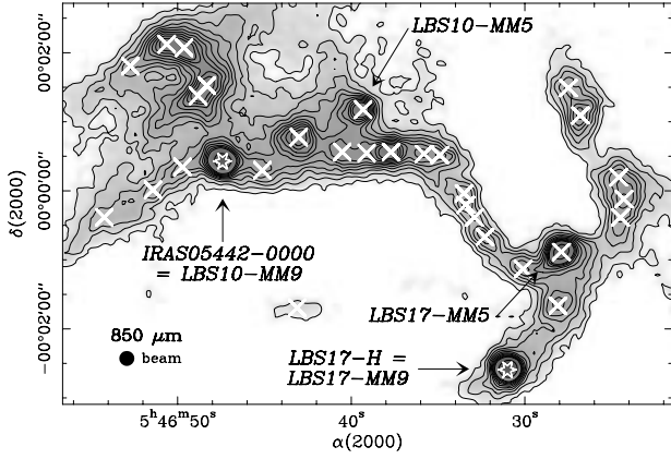
Fig. 2. Blow-up 850 \mu\text{m} continuum map of a sub-region around NGC 2068. The effective angular resolution is 13". Contour levels go from 65 to 650 mJy/beam with steps of 65 mJy/beam; last contour is 1 Jy/beam. The mean rms noise level is \sim 22 mJy/13"-beam. Starless condensations are denoted by crosses and embedded YSOs by star markers.
