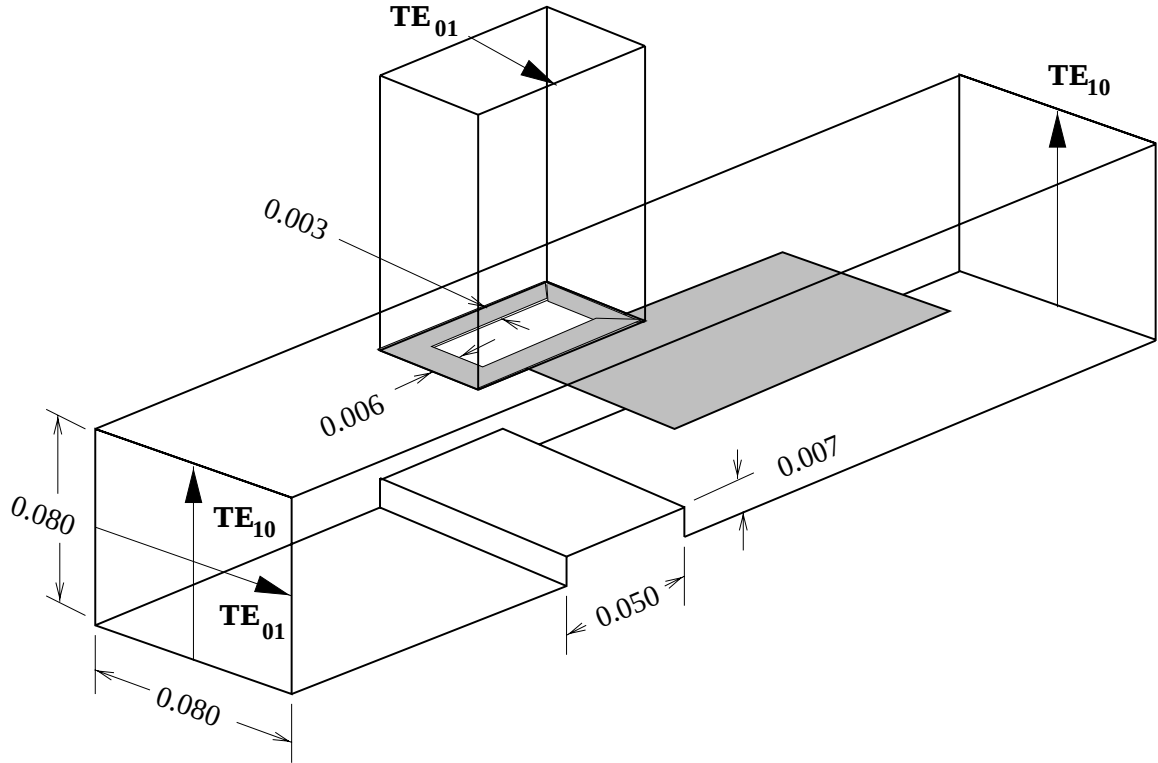
Figure 5.2 Detailed sketch of the Orthomode transducer. The dimensions are in inches.
