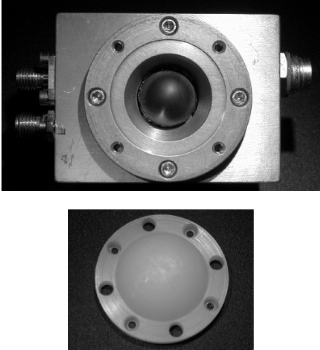
Figure 3.9 Actual picture of an assembled block, with the polyethylene lens removed to show the AR coated silicon hyperhemisphere. The SMA connectors for the two IF outputs can be seen on the left and the multi-pin bias connector can be seen on the right.
