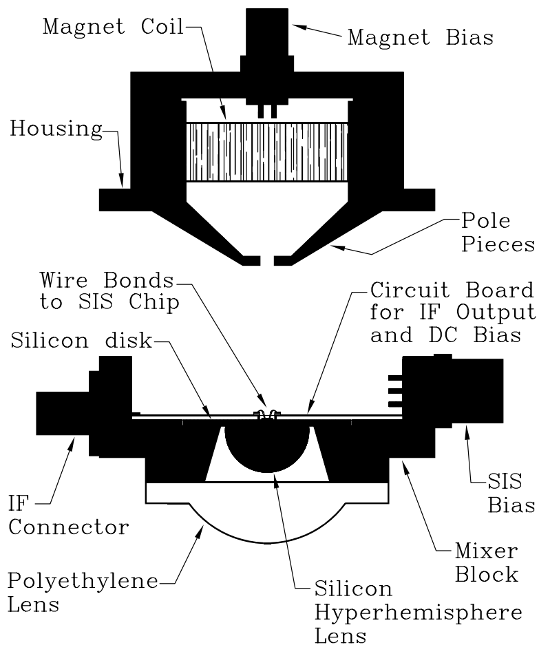
Figure 3.8 Schematic of the mixer block showing the hardwares used inside the block.
