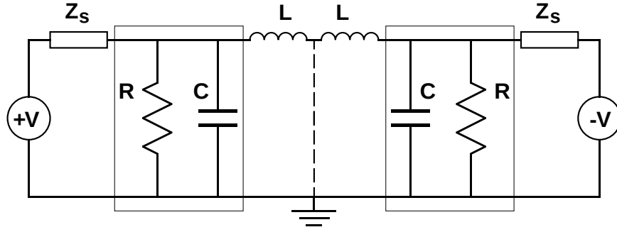
Figure 1.7 The equivalent circuit of the SIS mixer connected with the twin-slot antenna. The junctions can be idealized as simple parallel RC circuits. The physical spacing between the junctions determines the effective tuning inductance L . The slot antennas and microstrip transformers can be considered to be generators with complex source impedance Z_s ; the two generators are 180^\circ out of phase due to the symmetry of the circuit.
