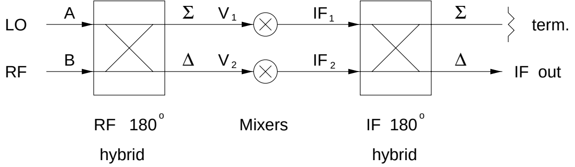
Figure 4.1 Circuit diagram of an ideal balanced mixer which uses 180° RF and IF hybrid circuits.
