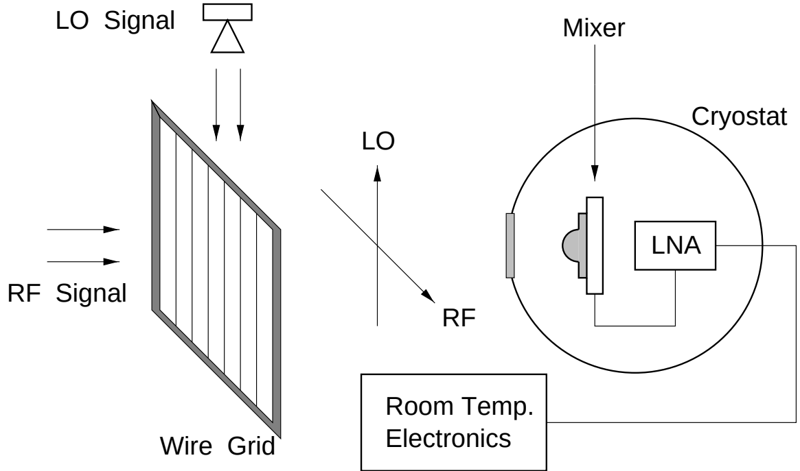
Figure 4.5 Measurement set-up for the balanced mixer. The LO frequency was 528 GHz and the cryostat temperature was 4.2 K.
