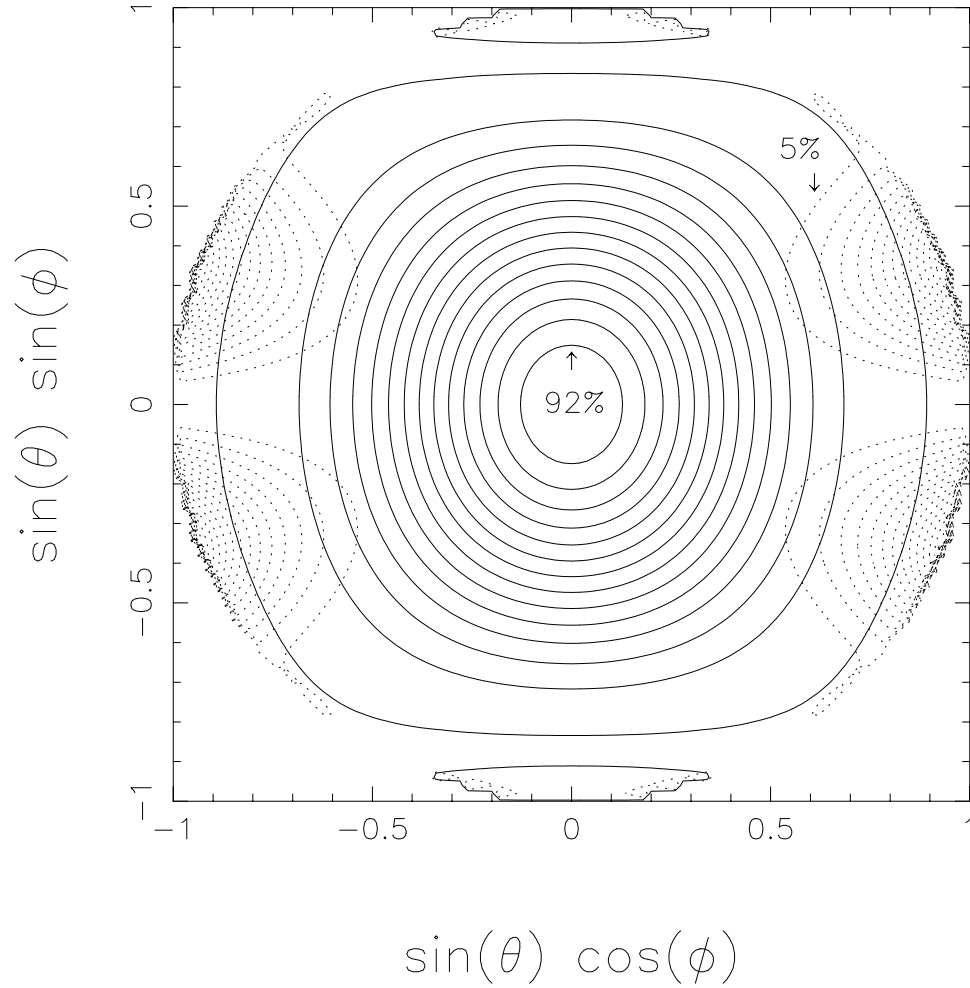
Figure 2.3 Contour plots of the calculated co-polarized and cross-polarized power pattern radiated into the dielectric by the antenna. The solid lines are for the co-polarized power and the dotted lines are for the cross-polarized power. The dimensions of the slot are the same as in Figure 2.2. For the co-polarized power, the contours are linearly spaced from 1% to 92% of the peak co-polarized power, in increments of 7%; and for the cross-polarized power, the contours are linearly spaced from 5% to 95% of the peak cross-polarized power in increments of 5%. The quantities (\theta, \phi) are the usual polar angles with respect to \hat{z} .
