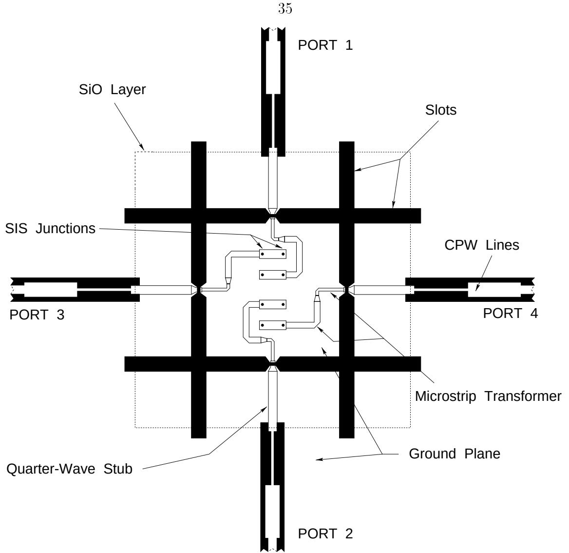
Figure 3.2 Details of the mixer layout. CPW lines carry the IF output to the 180^\circ hybrid, not shown here. The junctions are placed as shown to allow suppression of the Josephson effect with a single magnet.
