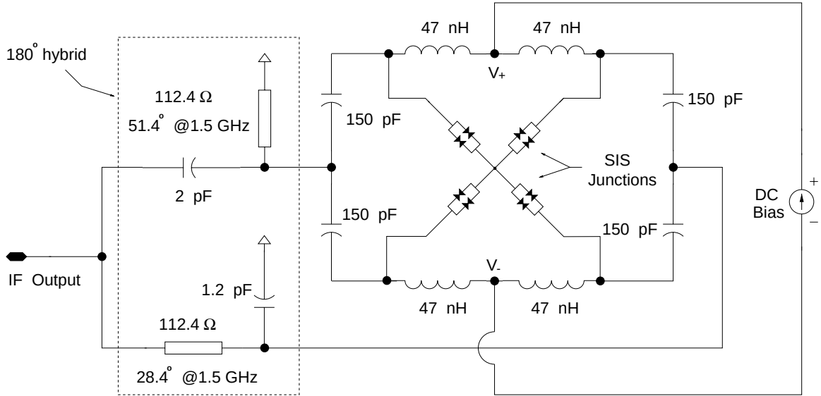
Figure 4.4 The details of the IF and DC bias circuits.
