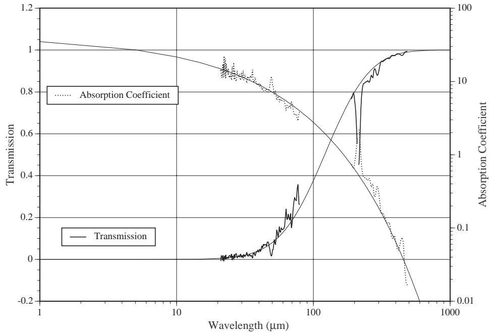
Fig. 7.— Transmission and absorption of Zitex G125.
