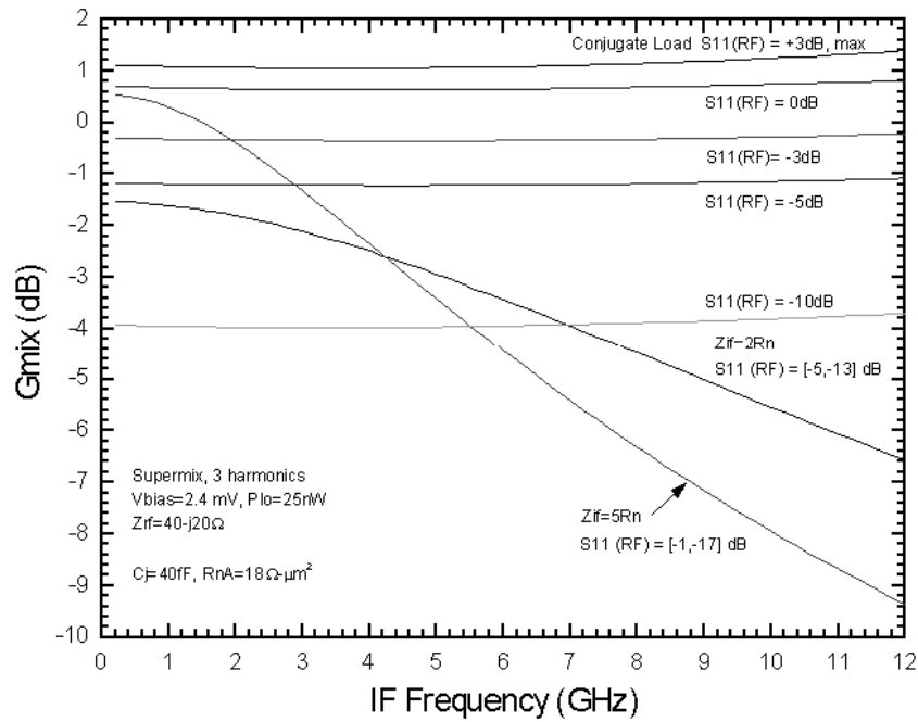
Fig. 5 Mixer gain and RF reflection, S_{11}(\text{RF}) , as a function of IF frequency for different IF loads. Presenting a conjugate load results in a mixer gain, but also a large RF reflection gain (+3dB)! Presenting a real load such as 2R_n or 5R_n is adequate at the lower IF frequencies, but results in a large loss in mixer performance at the higher IF frequencies.
