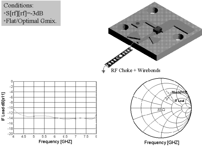
Fig. 7 A 4-8 GHz IF matching network which transforms a 50 Ohm input impedance to the required IF load impedance given the condition, S_{11}(\text{RF}) = -3\text{dB} . Since it is physically impossible to provide a negative capacitance, a good impedance match can only be provided over a limited (octave) of bandwidth.
