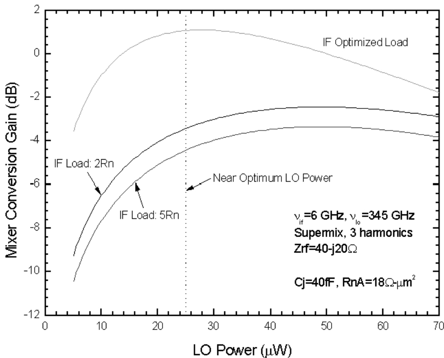
Fig. 10 LO Requirement for different IF port Impedances.
