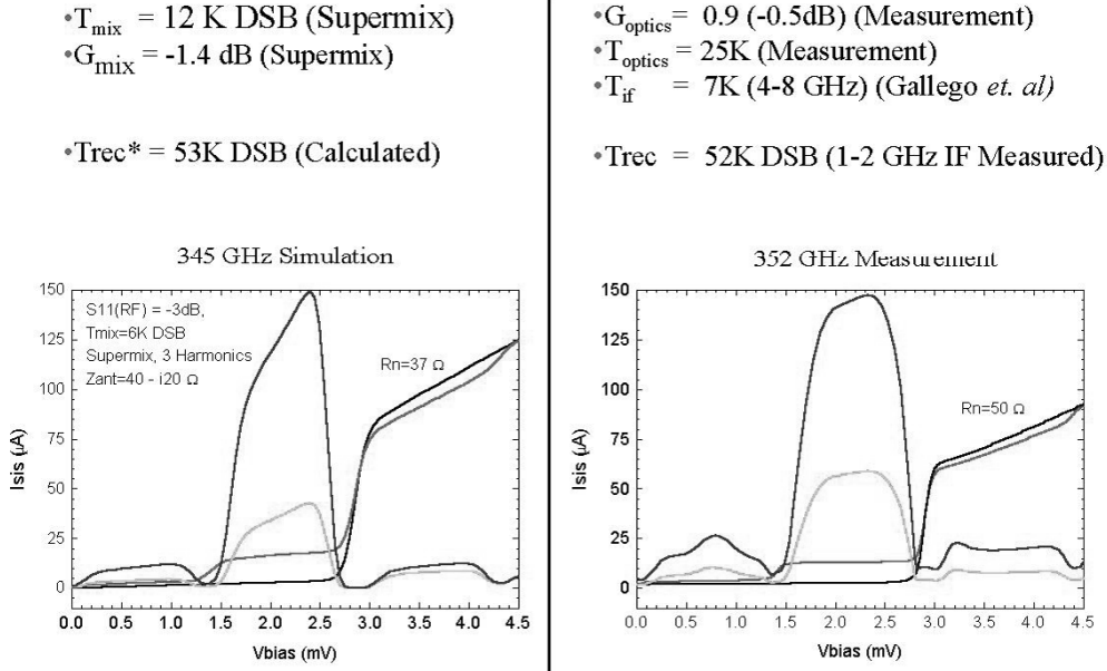
Fig. 9 To show that the simulations fit closely to actual measurements, we show this graph. The 352 GHz data was taken with a 1-2 GHz IF. The noise temperature of the LNA is about 5-6 K. The simulations assume a IF frequency of 6 GHz, but with similar IF noise characteristics. Material loss is measured in the lab and verified by the intersecting line technique (Blundell, Feldman et al ).
