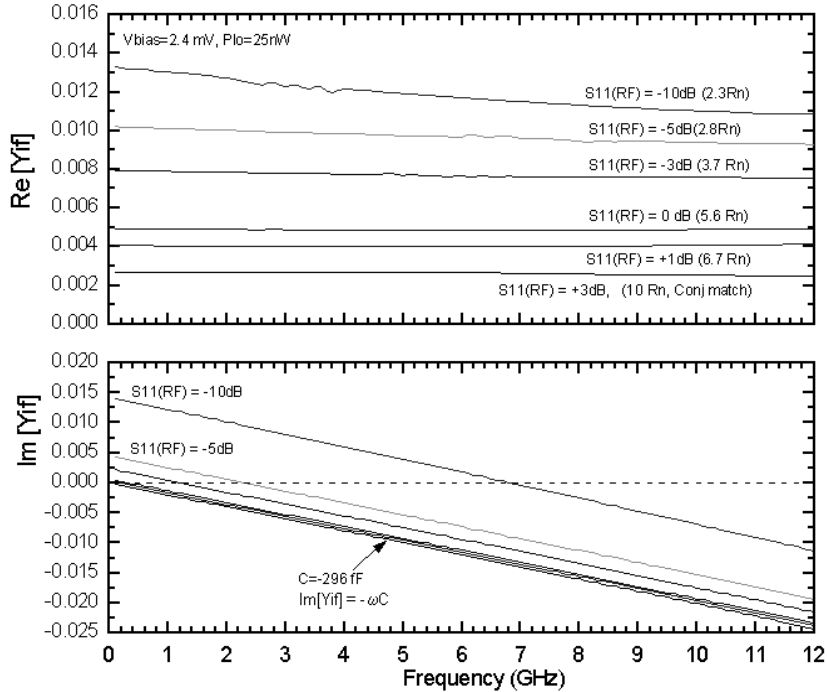
Fig. 6 IF load impedance required to obtain a fixed RF reflection Coefficient, S_{11}(\text{RF}) , and flat mixer gain. Note that a negative capacitance is required to achieve a good match over the whole IF frequency range.
