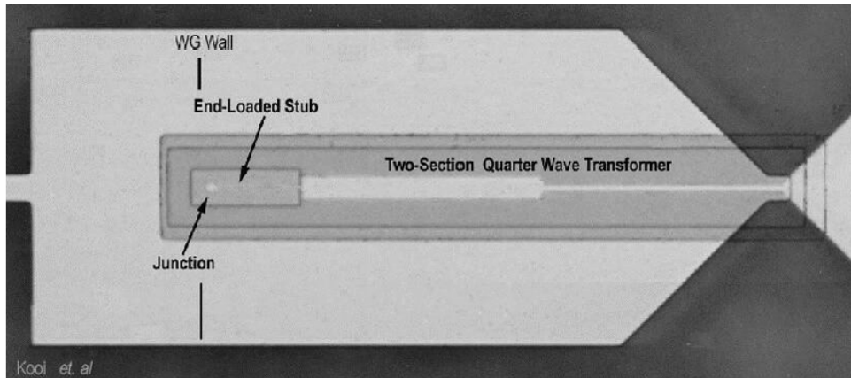
Fig. 1 End Loaded Stub RF matching Network and motivation for the work
