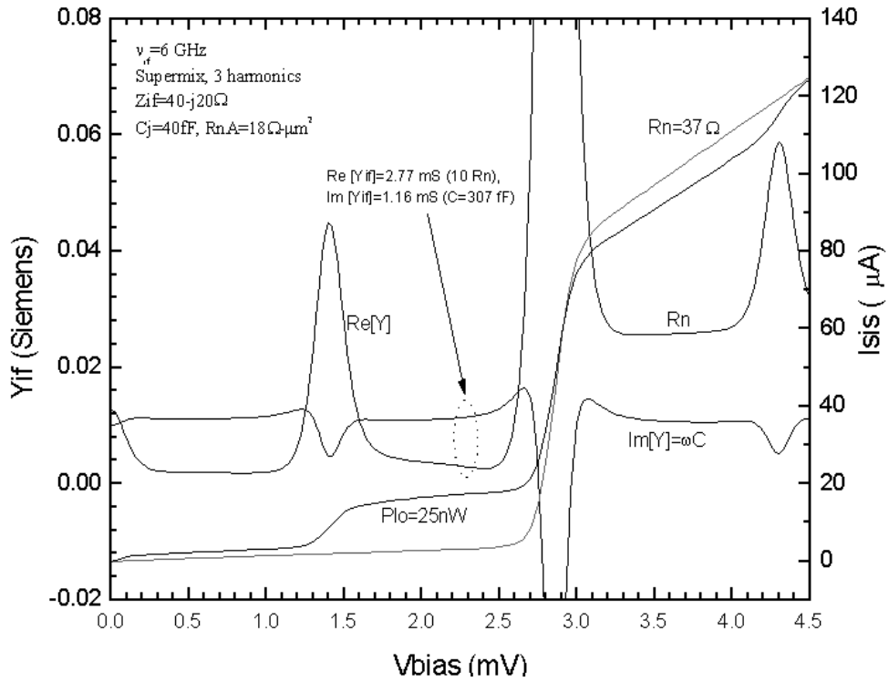
Fig. 3 345 GHz End-loaded stub IF output admittance. The real part of the IF impedance is close to 10R_n , while the imaginary part corresponds to a 307 fF capacitance. This capacitance is a combination of junction, RF choke and quantum susceptance.
