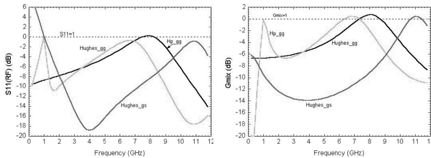
Fig. 12 Supermix computer simulations with the InP MMIC's connected to mixer IF port via a RF choke. That the IF load impedance presented by the MMIC to the mixer is far from ideal, is evident by the mixer gain and RF reflection, S11(RF). To take full advantage of the MMIC's very large IF bandwidth, the mixer will have to be redesigned so that the MMIC amplifier/RF choke combination provides an adequate termination to the mixer IF port (less capacitive RF matching network).
