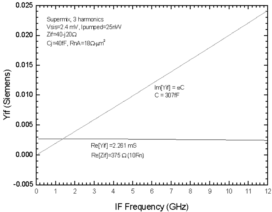
Fig. 4 End-loaded Stub IF output admittance as a function of IF frequency.
