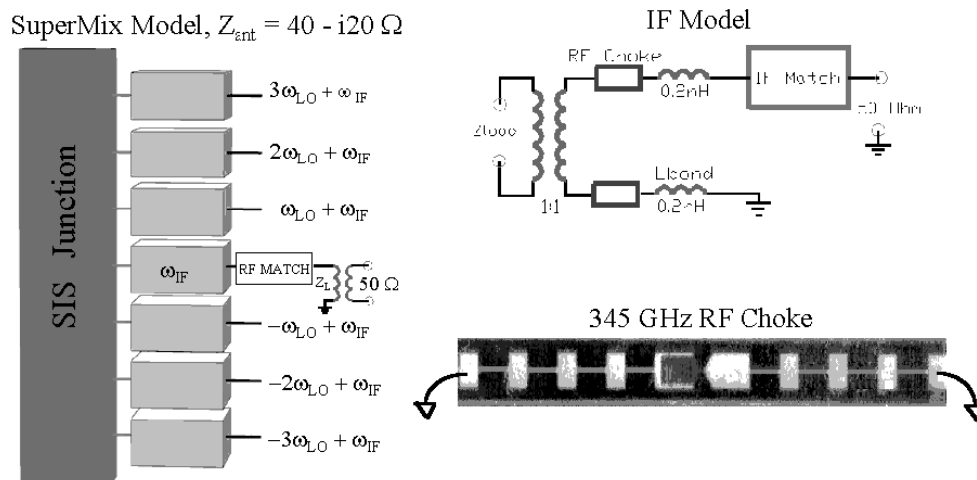
Fig. 2 Outline of the Computer Simulations. The Supermix mixer model assumes 3 harmonics for the harmonic balance. The Antenna impedance is taken to be 40-i20 Ohm. The IF model includes the RF choke and bond wires. A ideal transformer is used to obtain the load impedance at the junction/RF matching network, situated in the center of the Bowtie antenna.
