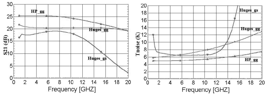
Fig. 11 InP MMIC computer simulations. Models obtained from Sander Weinreb. These simulations assume a fixed 50 Ohm input/output termination.
