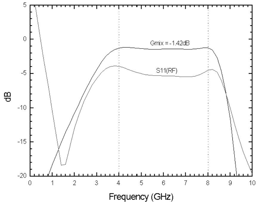
Fig. 8 The calculated IF load presented by the IF matching network and RF choke is now used to terminate the IF port of the mixer model. Supermix computer simulations are re-run, and the result for G_{\text{mix}} and S_{11}(\text{RF}) plotted.
