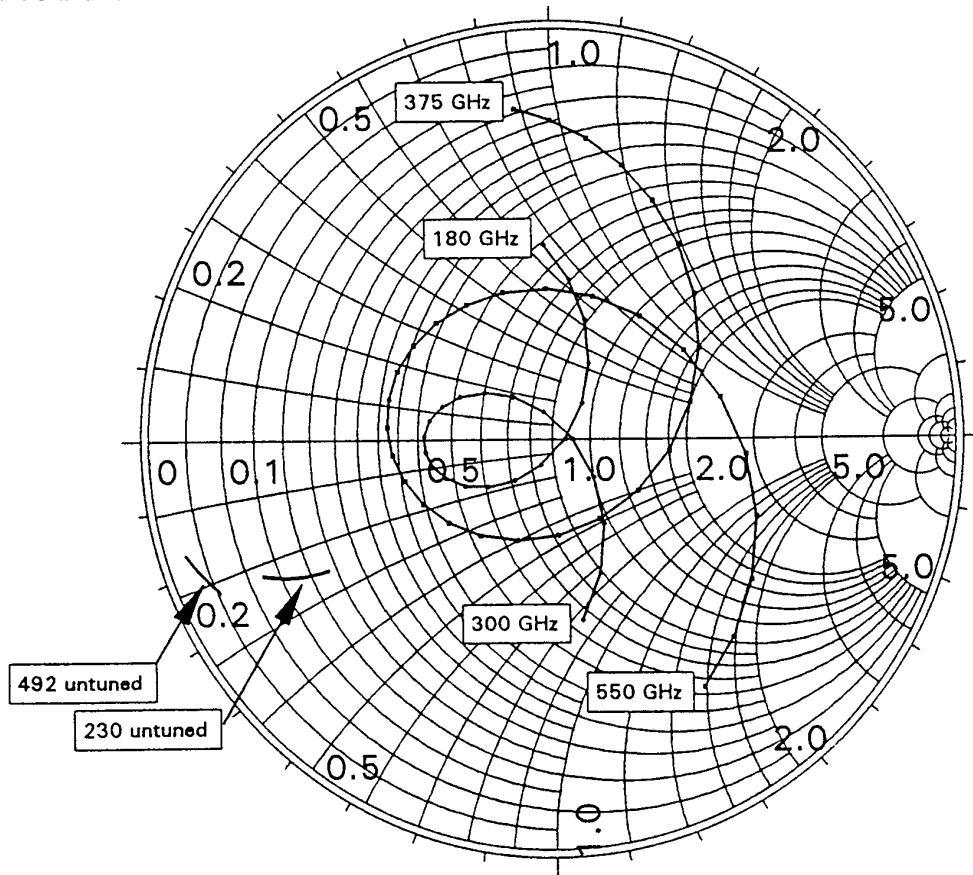
Figure 4. 230 GHz and 492 GHz tuned and untuned junction impedance plot normalized to 50 Ω. For the untuned junctions very high quality (Q) tuners are needed to tune out the probe impedance.
