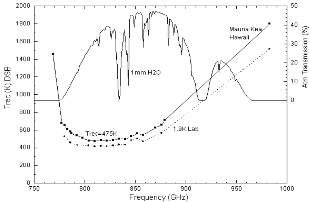
Figure 8. Frequency Response of the 850 GHz SIS receiver installed at the CSO. The receiver uses cooled (4K) optics to minimize the front end RF loss contribution. The mixer uses a Nb/ \text{AlO}_x /Nb SIS tunnel junction.
