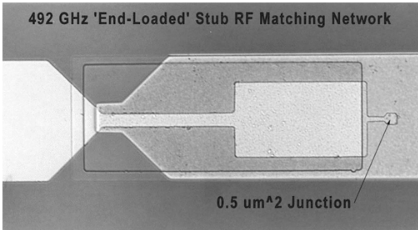
Figure 2. Physical layout of the 492 GHz SIS junction with an 'Endloaded Stub' RF matching network. The junction stub is fabricated on 150 nm thick \text{SiO} dielectric while the two section transformer is fabricated on a 450 nm thick \text{SiO} dielectric \text{SiO} ( \epsilon_r = 5.6 ). The junction is deposited inside a 5\mu\text{m} \times 5\mu\text{m} pad for alignment purposes.
