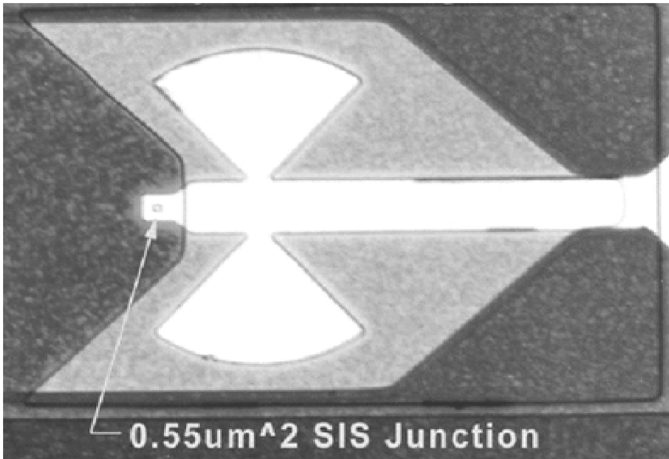
Figure 5. 1000 X photograph of the Nb/AlO x /Nb SIS junction and “Butterfly” RF matching network. The niobium transmission line and junction wiring are deposited on 450 nm and 200 nm dielectric of SiO respectively ( \epsilon_r = 5.6 ).
