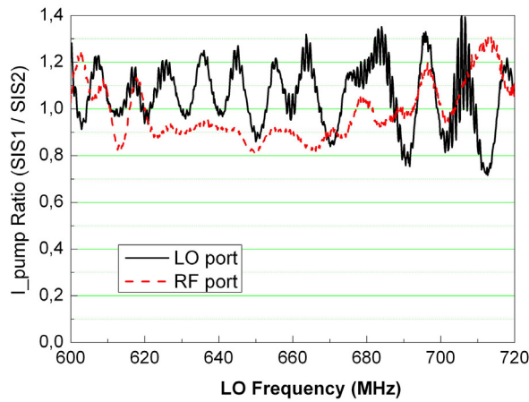
Figure 3. Ratio of pumping currents of the SIS junctions at the signal injection through the RF or LO ports.
