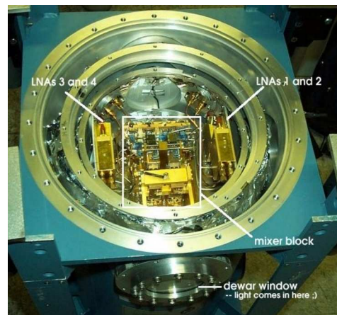
Figure 2: The inside of the PoleStar cryostat.
