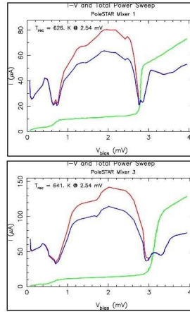
Figure 4: Post-upgrade IV and total power curves from the three functioning mixers.
