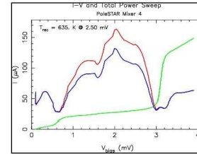
PoleSTAR IV & Total Power Curves
