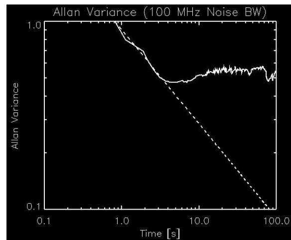
Figure 12: An Allan variance plot from 160 minutes of total power data taken every 50 ms.
