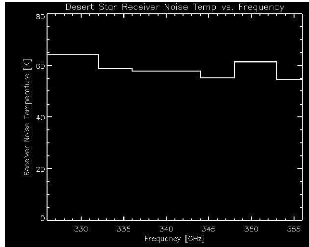
Figure 11: Receiver noise temperature (Mixer 1) as a function of LO frequency.
