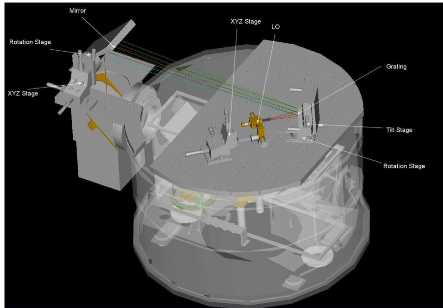
Figure 8: A cutaway CAD drawing of DesertStar.
