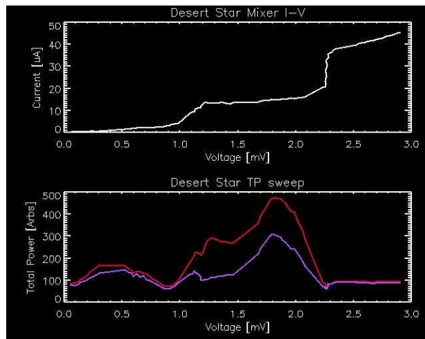
Figure 10: Representative IV and hot/cold total power curves.
