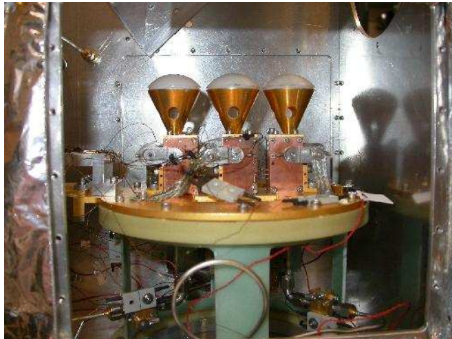
Figure 9: A photograph of three mixers installed in the JT cryostat before testing.
