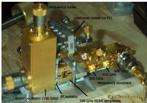
Figure 3: The JPL/UMass LO chain added to PoleStar.
