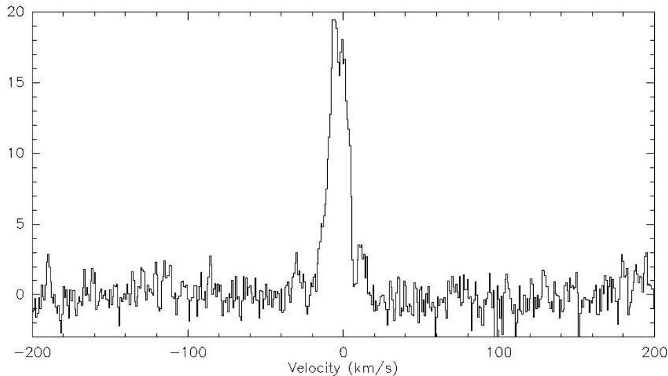
Figure 7: ^{12}\text{CO} (3-2) Spectrum from the central position of a map of the high mass star forming region DR21.
